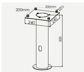
Art. 117 3101929 Markfeste Asker stolpe
