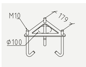
Art. 405 3183055 Festejern Stockholm Oslo Lund Rimini/Milano Koster Lofoten
