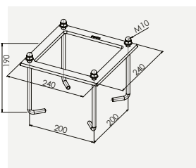
Art. 116 3110095 Festejern Asker stolpe
