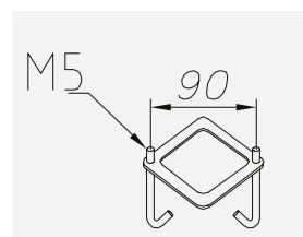
Art. 307 3185231 Festejern Chelsea Bologna London Modena
