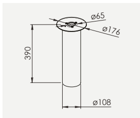
Art. 6133 3101980 Adapter for betongfundament.
