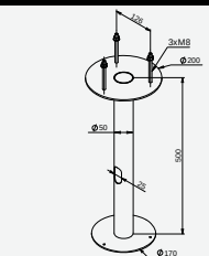
Art. 1230 Concreting anchor Stavanger Egersund
