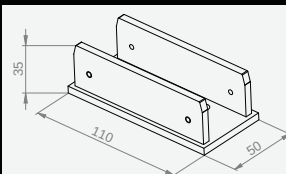
Art. 1906 Reinforced galvanized metal foot for Molde
