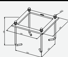
Art. 113 Anchoring support Namsos
