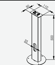
Art. 1907 Concreting anchor Molde Asker bollard
