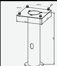
Art. 116 Concreting anchor Asker pole
