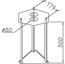
Art. 405 Concreting anchor Art: 242 Art: 274, 275 Art: 281, 283 Art: 401, 402, 403 Art: 1914 Lofoten
