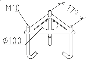
Art. 405 Concreting anchor Art: 242 Art: 274, 275 Art: 281, 283 Art: 401, 402, 403 Art: 1914 Lofoten
