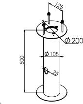
Art. 1230 Concreting anchor Art: 1240, 1243, 1244, 1246, 1248, 1248 Art: 1280, 1285
