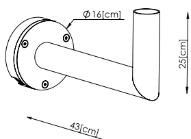
Art. 154 Fixation murale Ø60 Asker Head Borg Hammerfest Mora Visby
