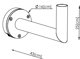
Art. 154 Fixation murale Ø60 Borg Hammerfest Visby
